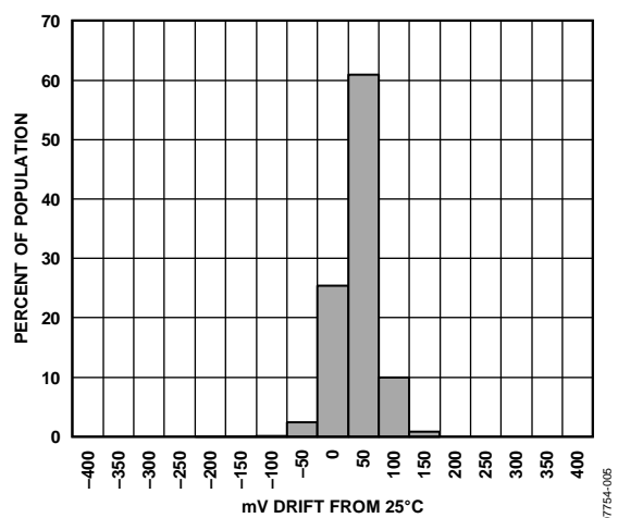
Figure 5. Null Drift over Temperature ( V_{RATIO} = 5\text{ V} )
