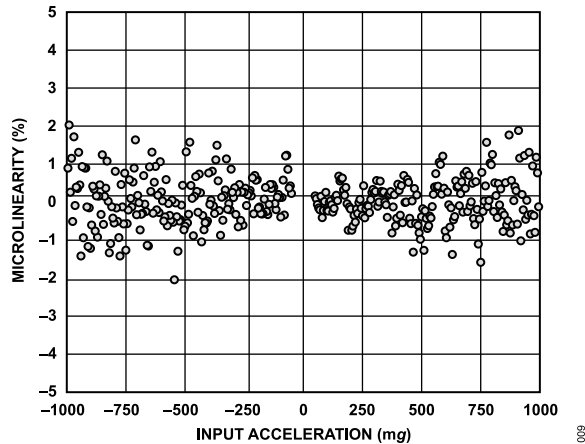
Figure 10. X-Axis Microlinearity, 50 mg Step Size
