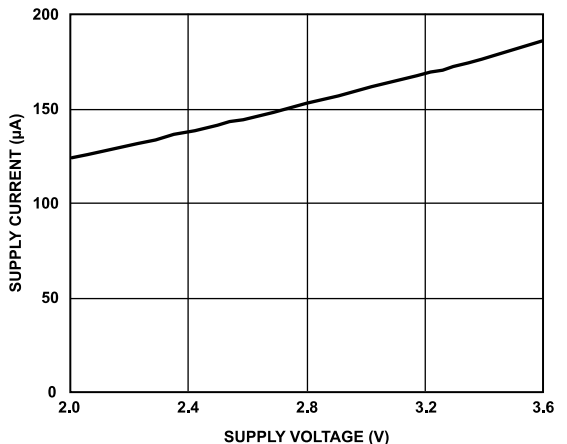
Figure 15. Supply Current vs. Supply Voltage, V_S at 25^\circ\text{C}
