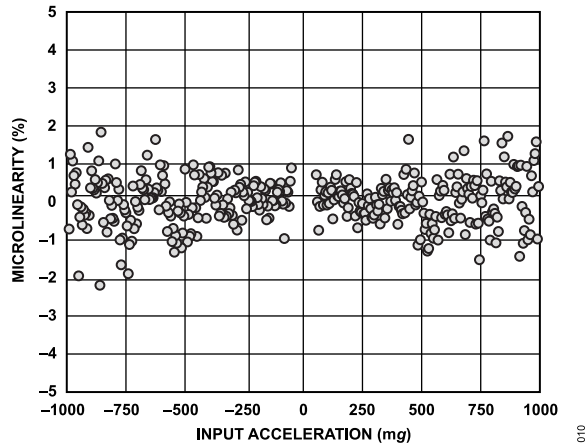
Figure 11. Y-Axis Microlinearity, 50 mg Step Size
