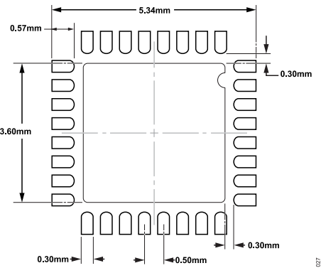
Figure 31. Sample Solder Pad Layout (Land Pattern)
