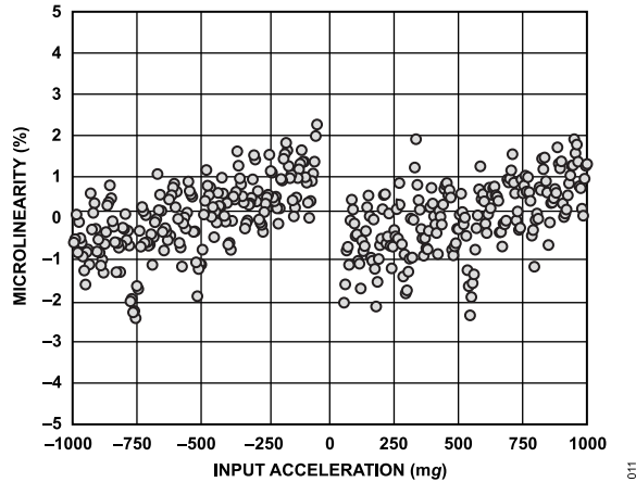
Figure 12. Z-Axis Microlinearity, 50 mg Step Size
