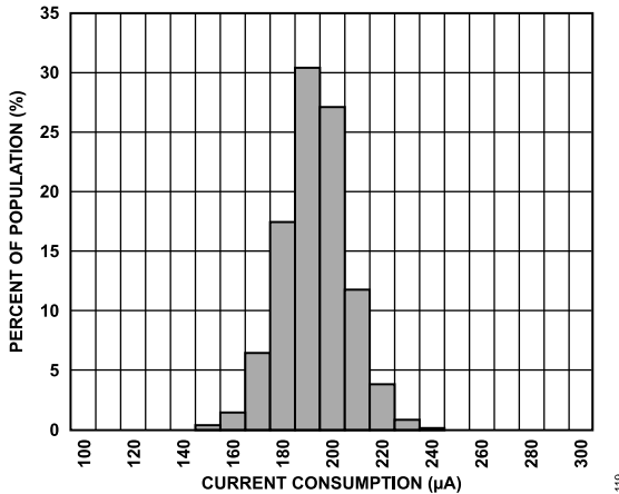
Figure 14. Current Consumption, Measurement Mode, Data Rate = 100 Hz, V_S = V_{DD\ I/O} = 3.3\text{ V} , 25^\circ\text{C}
