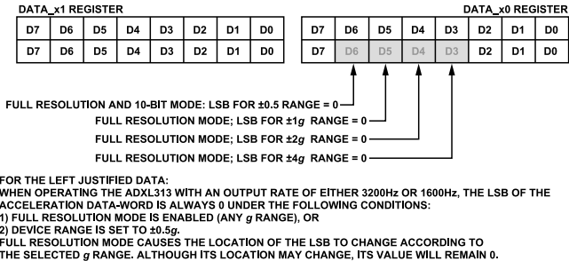
Figure 27. Left Justified Data Formatting: 3200 Hz and 1600 Hz Output Data Rate
