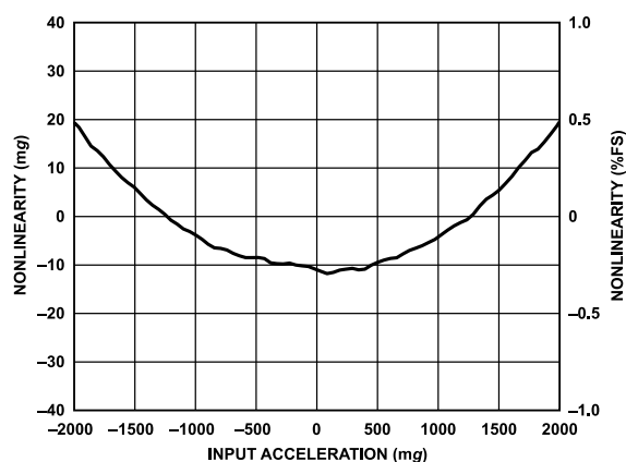
Figure 9. Z-Axis Nonlinearity, \pm 2 g Input Range
