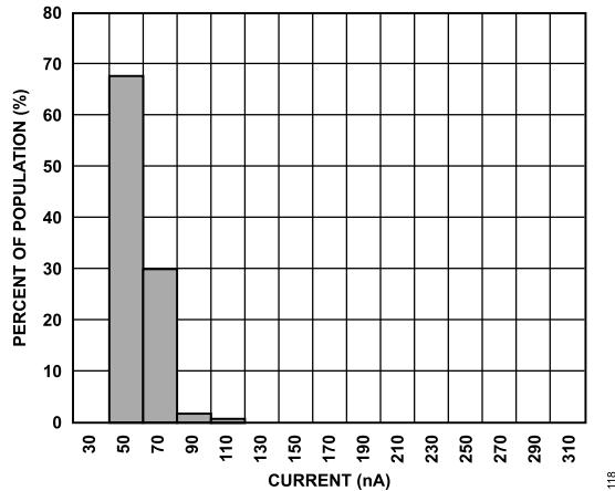
Figure 13. Standby Mode Current Consumption, V_S = V_{DD\ I/O} = 3.3\text{ V} , 25^\circ\text{C}
