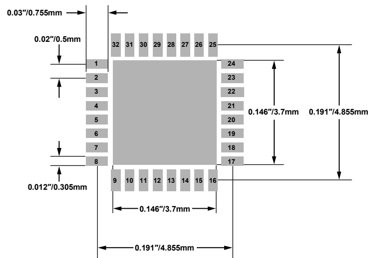
Figure 25. PCB Land Pattern
