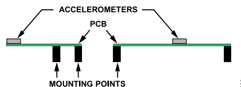
Figure 27. Incorrectly Placed Accelerometers
