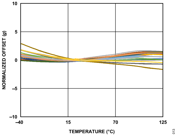
Figure 13. ADXL1002 Normalized Offset vs. Temperature
