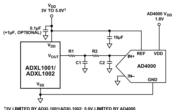
Figure 25. Application Circuit for the ADXL1001/ADXL1002
