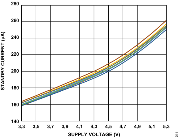
Figure 11. ADXL1001/ADXL1002 Standby Current vs. Supply Voltage
