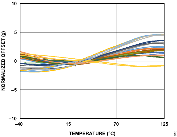
Figure 10. ADXL1001 Normalized Offset vs. temperature
