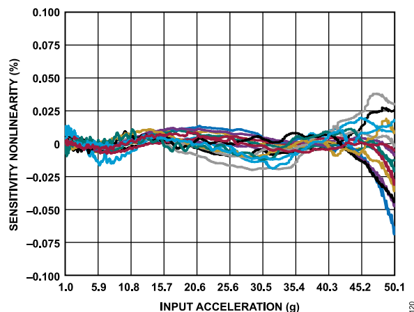
Figure 20. ADXL1002 Sensitivity Nonlinearity vs. Input Acceleration
