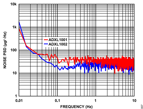
Figure 7. ADXL1001/ADXL1002 Noise Power Spectral Density (Noise PSD) Below 10 Hz
