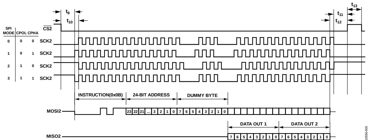
Figure 5. Detailed SPI Master Timing Diagram (Serial Port 2)
