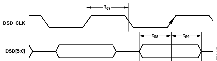
Figure 28. DSD Timing
