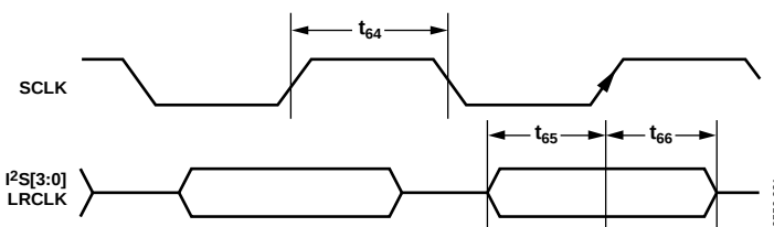
Figure 22. I²S Timing
