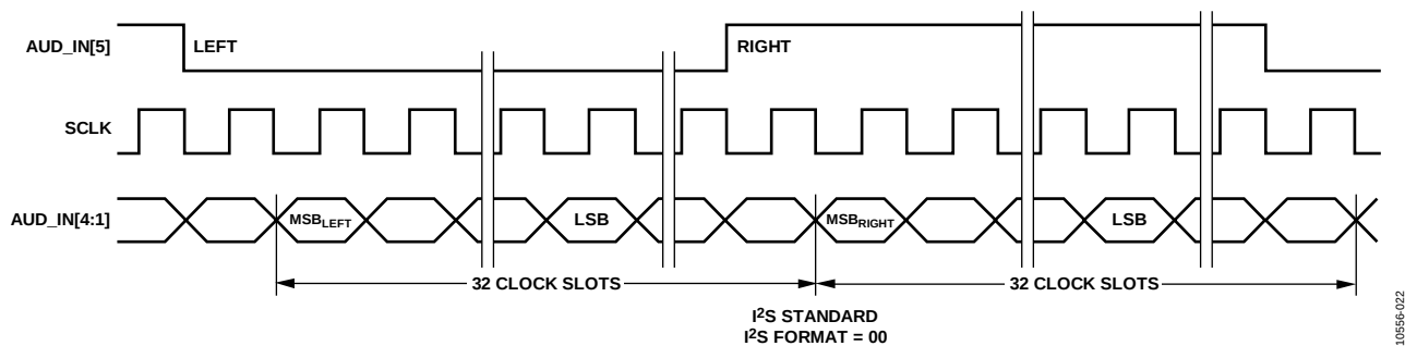
Figure 23. I²S Standard Audio—Data Width of 16 Bits to 24 Bits per Channel
