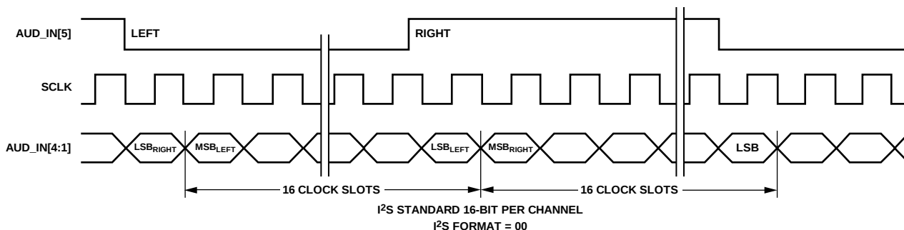
Figure 24. I²S Standard Audio—16-Bit Samples Only
