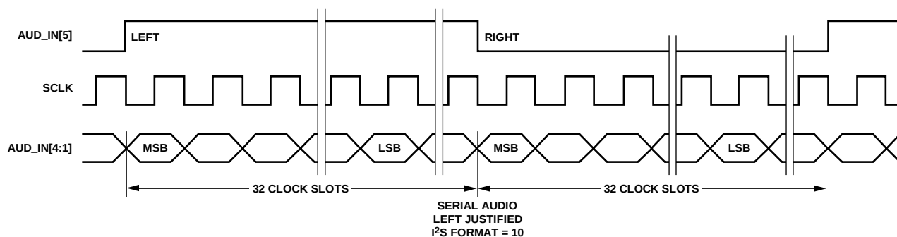
Figure 26. Serial Audio—Left-Justified
