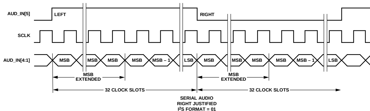
Figure 25. Serial Audio—Right-Justified
