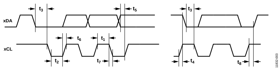
Figure 3. I²C Timing
