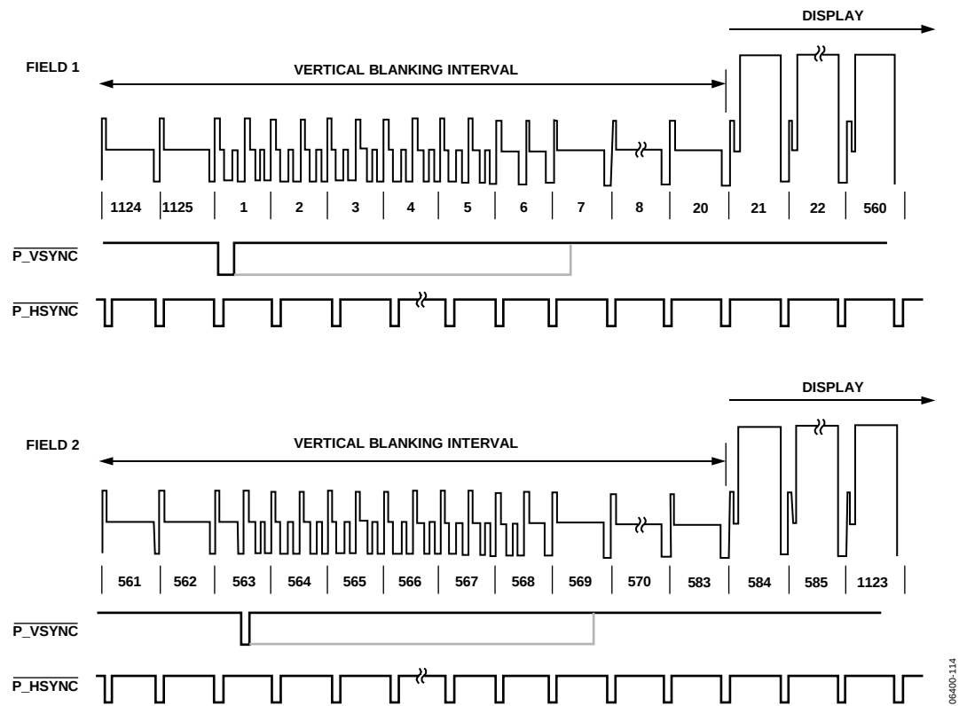
Figure 111. 1080i \overline{\text{HSYNC}} and \overline{\text{VSYNC}} Input Timing
