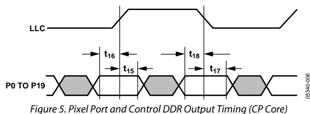
Figure 5. Pixel Port and Control DDR Output Timing (CP Core)
