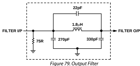
Figure 79. Output Filter
