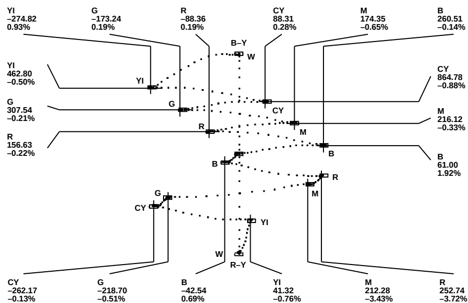
Figure 98. PAL YUV Lighting Plot
