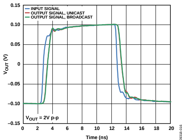
Figure 15. ADV3228 Large Signal Pulse Response
