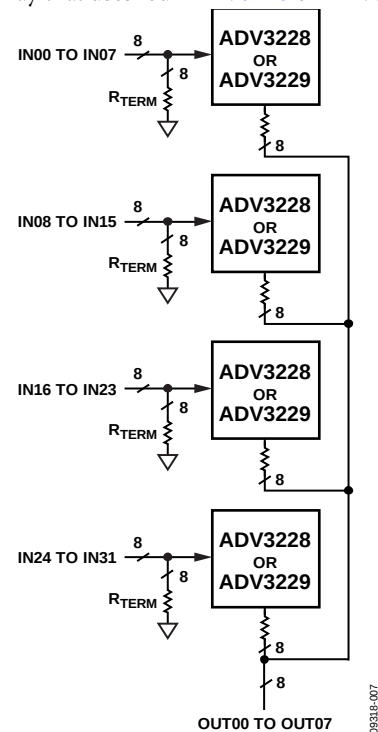
Figure 65. A 32 × 8 Nonblocking Crosspoint Switch Array
