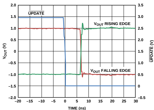
Figure 42. ADV3229 Switching Time
