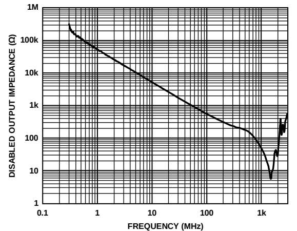
Figure 46. ADV3222 Disabled Output Impedance
