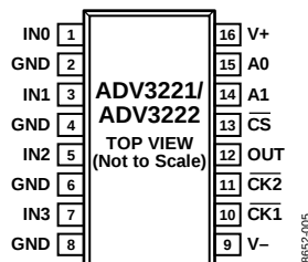
Figure 5. Pin Configuration
