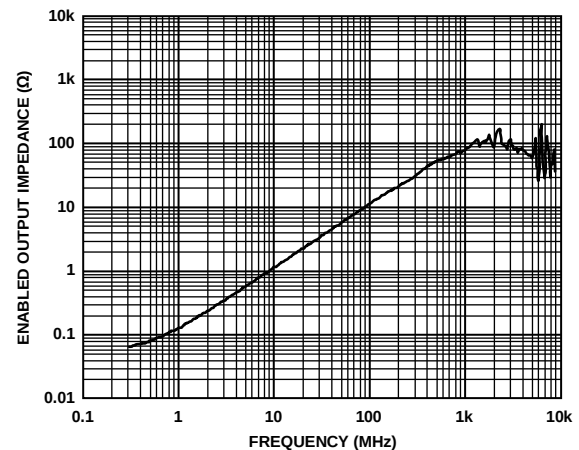
Figure 47. ADV3222 Enabled Output Impedance
