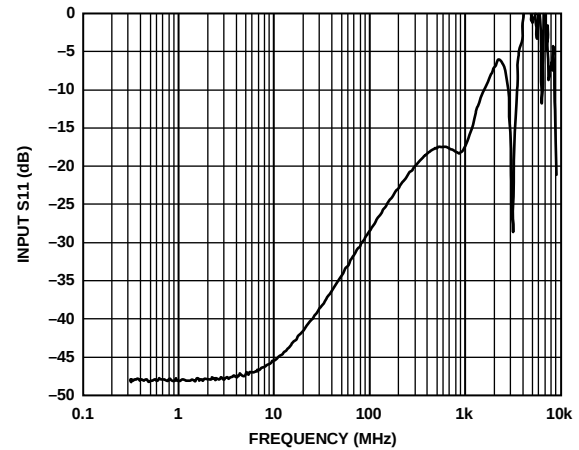
Figure 45. ADV3221/ADV3222 S11 (Including Evaluation Board)
