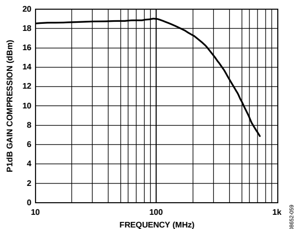
Figure 53. ADV3222 Output P1dB, R_L = 100\ \Omega , C_L = 4\ \text{pF}
