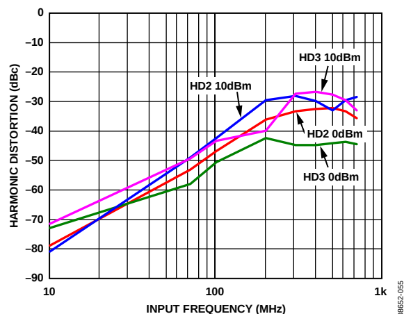
Figure 49. ADV3222 Harmonic Distortion, R_L = 100\ \Omega , C_L = 4\ \text{pF}
