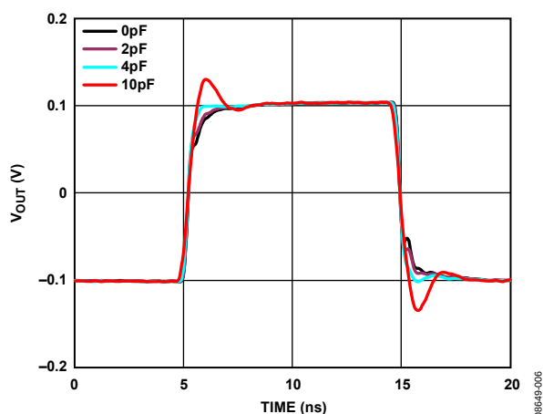
Figure 6. ADV3219 Small Signal Pulse Response vs. Capacitive Load, 200 mV p-p Output
