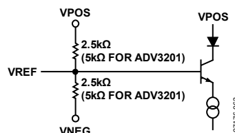
Figure 15. VREF Input (See Also Figure 16)
