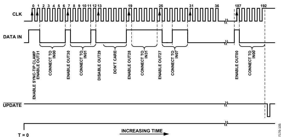
Figure 3. Programming Example
