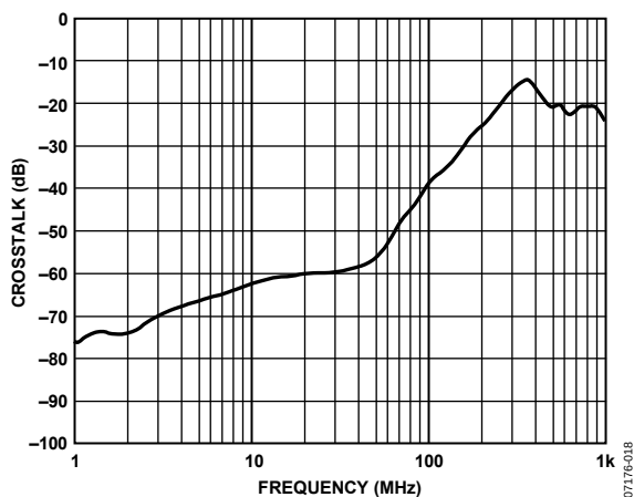
Figure 28. ADV3200 Crosstalk, One Adjacent Channel, RTO
