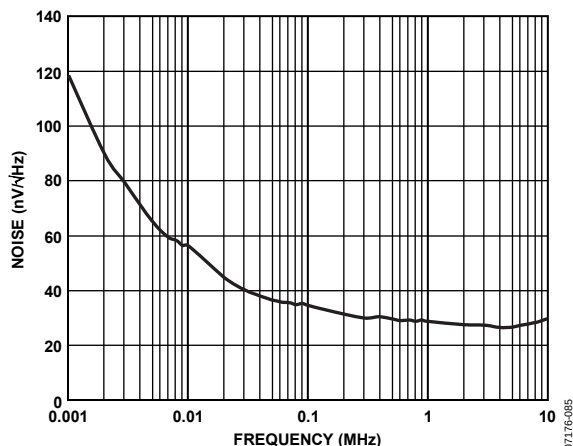
Figure 27. ADV3200 OSD Output Noise
