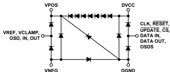
Figure 16. ESD Protection Map
