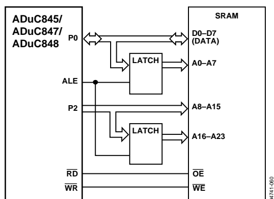
Figure 63. External Data Memory Interface (16-Mbyte Address Space)
