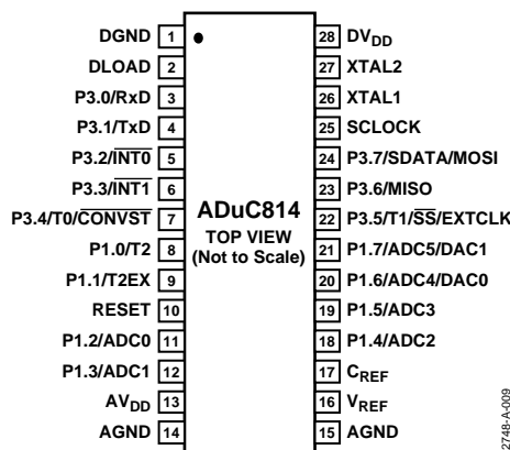
Figure 2. Pin Configuration
