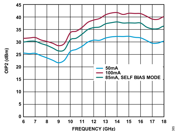
Figure 85. OIP2 vs. Frequency for Various I_{DQ\_LNA} , P_{OUT}/Tone = 0\text{ dBm} , Receive State, Path = ANT to RX_OUT, Self Biased Mode, VDD\_LNA = 3.3\text{ V} , Controlled VGG\_LNA , Transmit State Off
