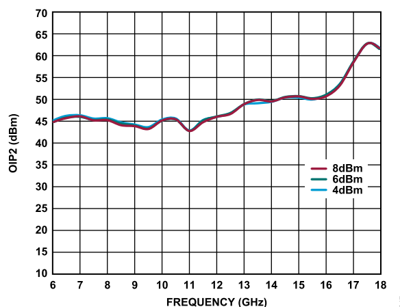
Figure 47. OIP2 vs. Frequency for Various P_{OUT}/Tone , Transmit State, Path = TX_IN to ANT, VDD_{PA} = 5\text{ V} , I_{DQ\_PA} = 220\text{ mA} , Receive State Off
