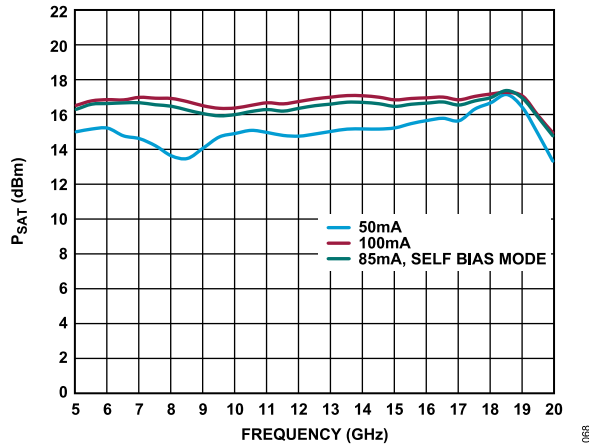
Figure 68. P_{SAT} vs. Frequency for Various I_{DD\_LNA} , Receive State, Path = ANT to RX_OUT, Self Biased Mode, V_{DD\_LNA} = 3.3 V, Controlled V_{GG\_LNA} , Transmit State Off
