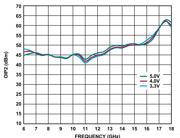
Figure 46. OIP2 vs. Frequency for Various VDD_{PA} , P_{OUT}/Tone = 8\text{ dBm} , Transmit State, Path = TX_IN to ANT, I_{DQ\_PA} = 220\text{ mA} , Receive State Off
