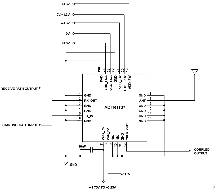
Figure 89. Typical Application Circuit
