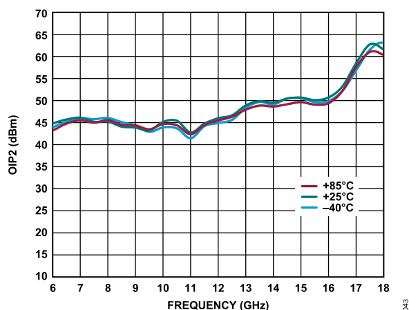
Figure 43. Output Second-Order Intercept (OIP2) vs. Frequency for Various Temperatures, P_{OUT}/Tone = 8\text{ dBm} , Transmit State, Path = TX_IN to ANT, VDD_{PA} = 5\text{ V} , I_{DQ\_PA} = 220\text{ mA} , Receive State Off
