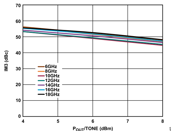
Figure 45. Third-Order Intermodulation Distortion Relative to Carrier (IM3) vs. P_{OUT}/Tone , Transmit State, Path = TX_IN to ANT, VDD_{PA} = 5\text{ V} , I_{DQ\_PA} = 220\text{ mA} , Receive State Off
