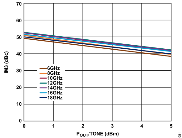
Figure 81. IM3 vs. P_{OUT}/Tone , Receive State, Path = ANT to RX_OUT, Self Biased Mode, VDD\_LNA = 3.3\text{ V} , VGG\_LNA = 0\text{ V} , Transmit State Off
