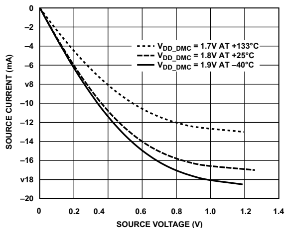
Figure 89. Driver Type B and Driver Type C (DDR2 Drive Strength 60 \Omega )
