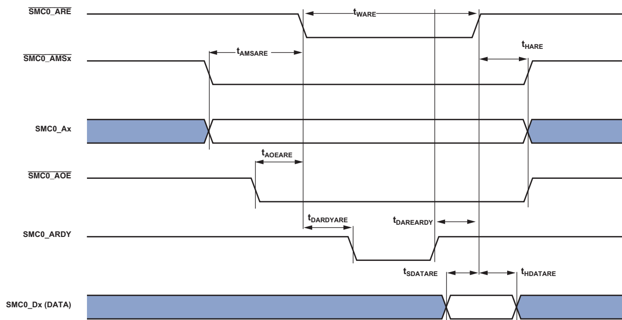
Figure 11. Asynchronous Read
