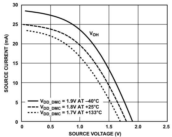
Figure 77. Driver Type B and Driver Type C (DDR2 Drive Strength 40 \Omega )
