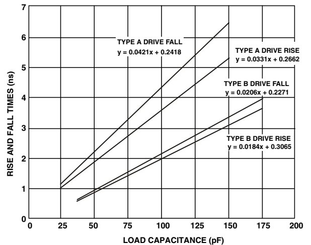
Figure 49. Typical Output Rise/Fall Time (20% to 80%, V_{DD\_EXT} = \text{Max} )
