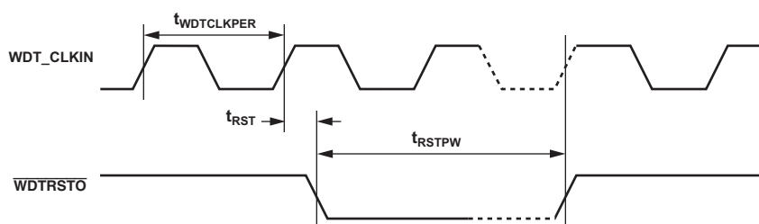
Figure 14. Watchdog Timer Timing
