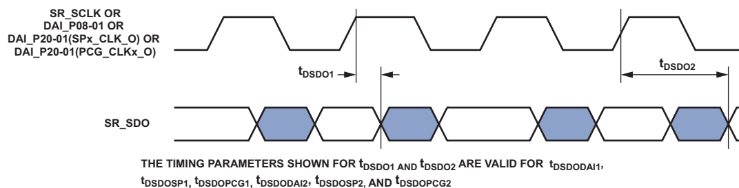
Figure 41. SR_SDO Delay
