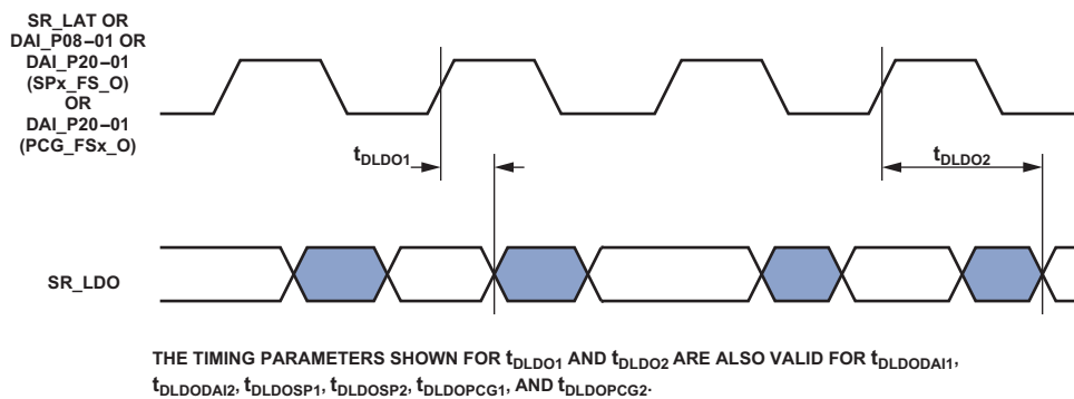
Figure 42. SR_LDO Delay
