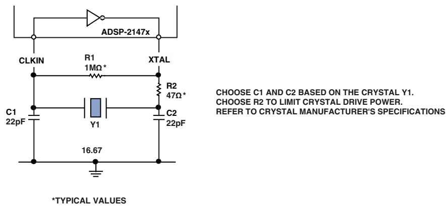
Figure 7. 266 MHz Operation (Fundamental Mode Crystal)
