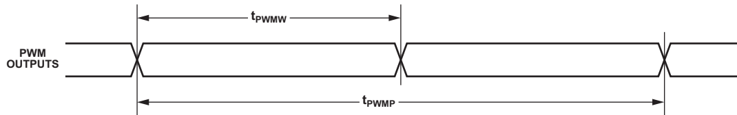
Figure 29. PWM Timing
