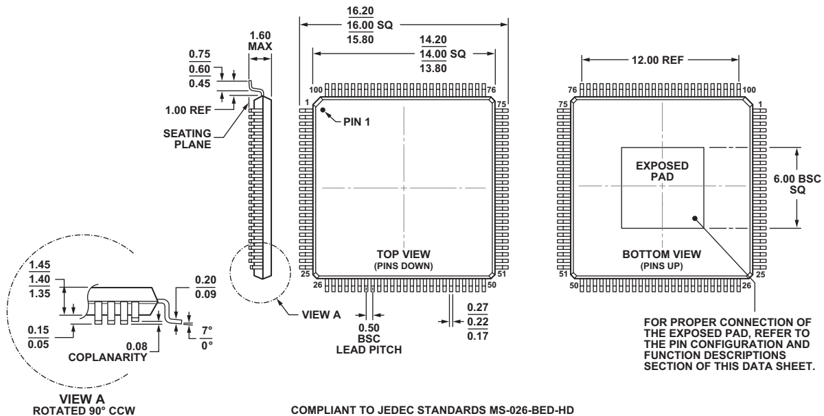
Figure 57. 100-Lead Low Profile Quad Flat Package, Exposed Pad [LQFP_EP¹] (SW-100-2)
