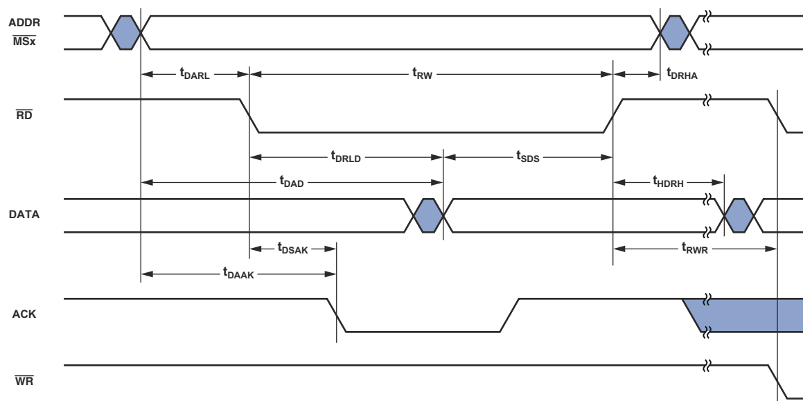
Figure 19. AMI Read
