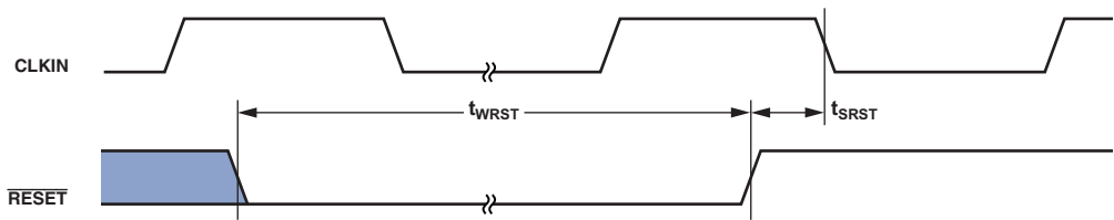
Figure 8. Reset
