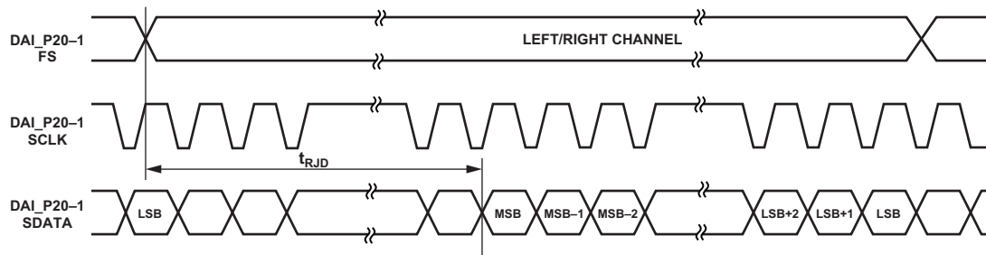
Figure 30. Right-Justified Mode
