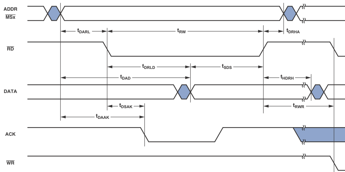
Figure 18. Memory Read
