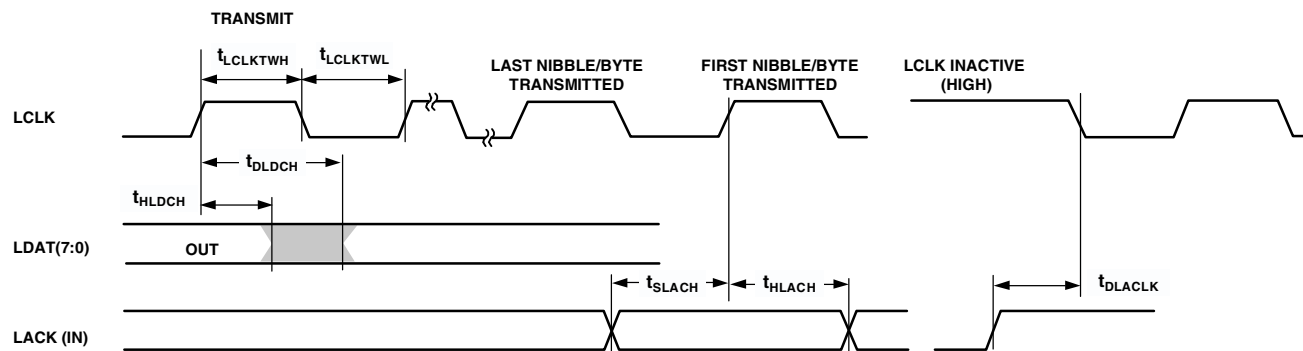
Figure 25. Link Ports—Transmit
