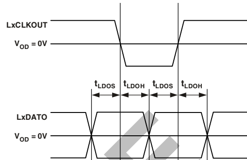
Figure 18. Link Ports—Data Output Setup and Hold 1
