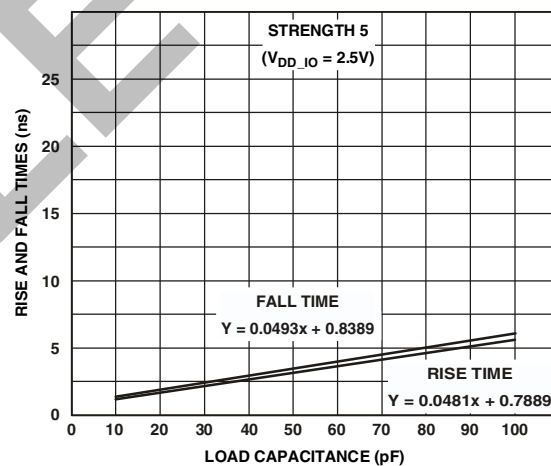
Figure 40. Typical Output Rise and Fall Time (10% to 90%, V_{DD\_IO} = 2.5V ) vs. Load Capacitance at Strength 5
