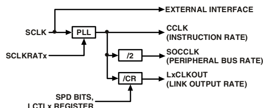
Figure 5. Clock Domains
