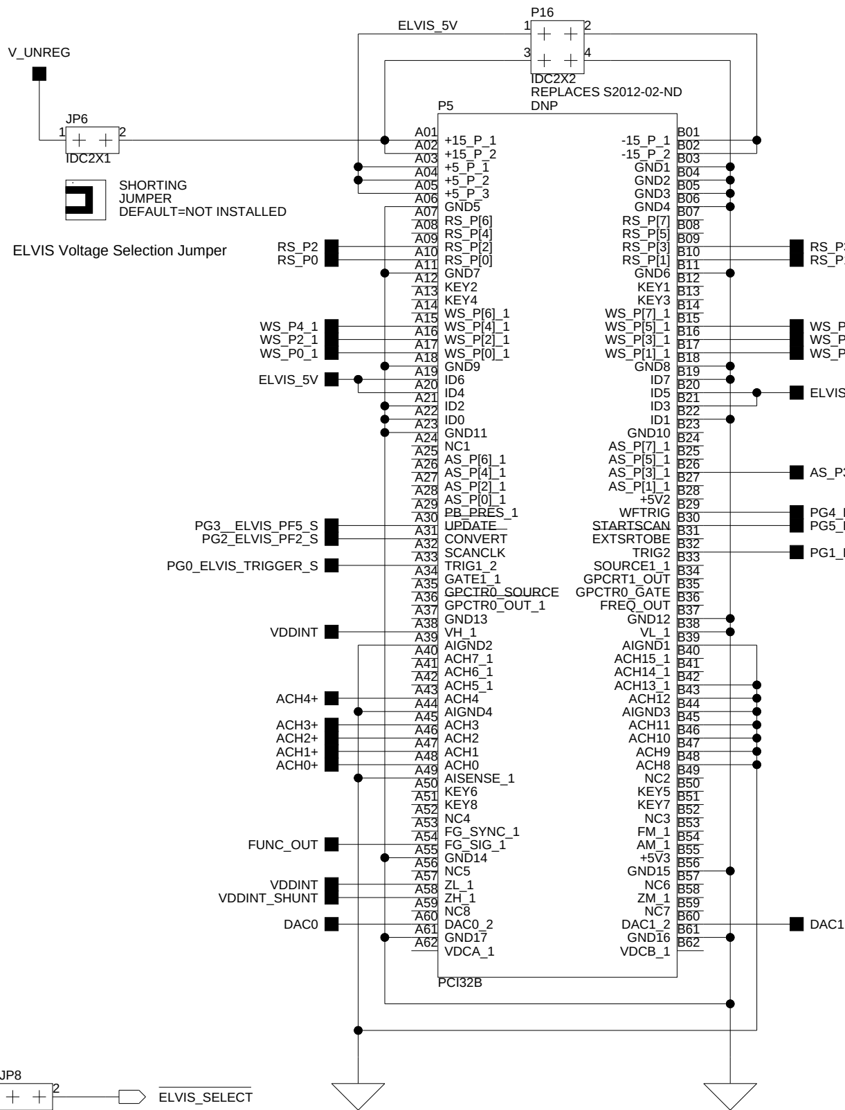
ELVIS CONNECTOR
