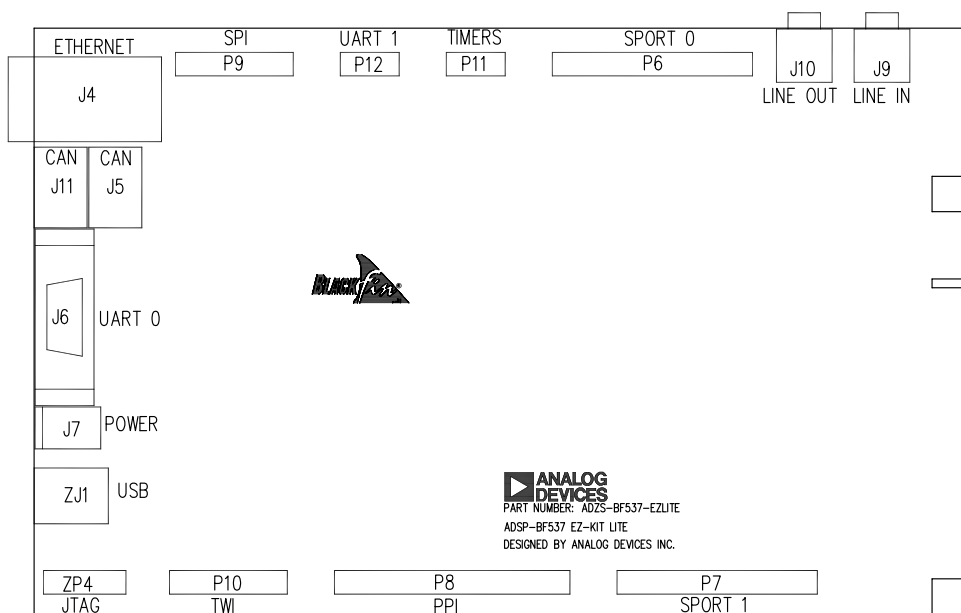
Figure 2-4. Connector Locations
