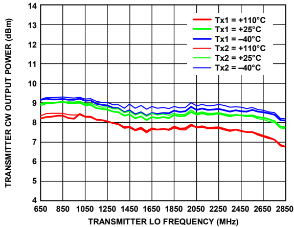
Figure 129. Transmitter CW Output Power vs. Transmitter LO Frequency, Transmitter QEC and External LO Leakage Active, Transmitter in 200 MHz/450 MHz Bandwidth Mode, IQ Rate = 491.52 MHz, 0 dB Attenuation, Not De-Embedded
