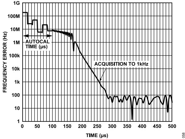
Figure 58. PLL Acquisition
