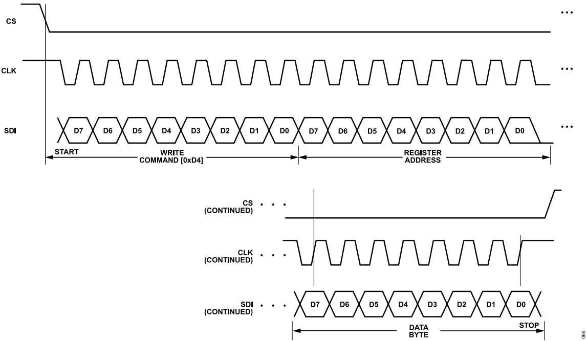
Figure 66. SPI Byte Write Example
