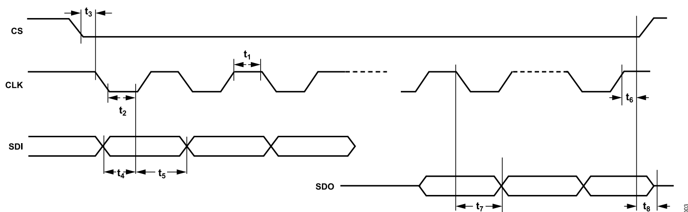
Figure 3. SPI Port Timing Diagram
