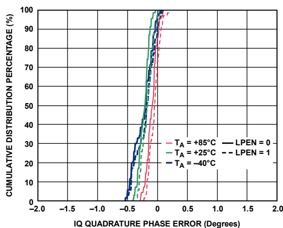
Figure 32. IQ Quadrature Phase Error
