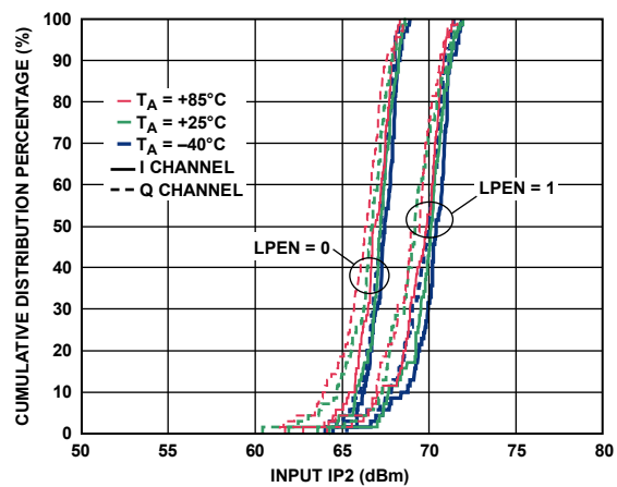
Figure 30. Input IP2
