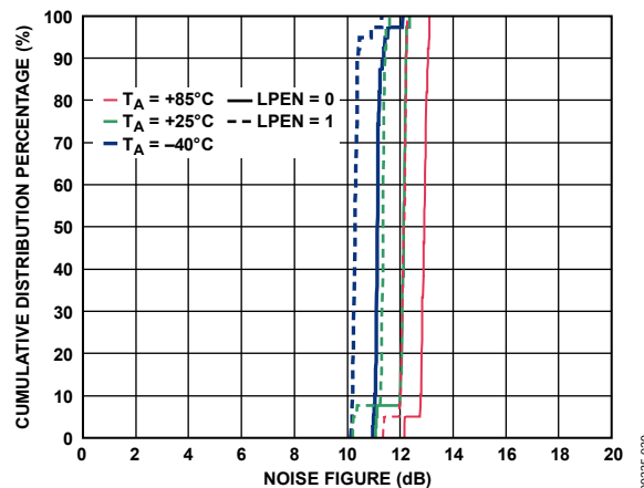
Figure 31. Noise Figure
