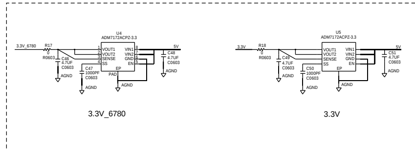
Figure 85. ADRF6780 Evaluation Board Schematic Page 3
