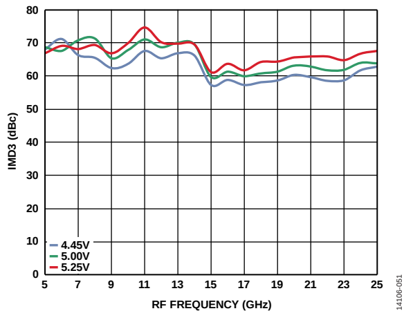
Figure 45. Third-Order Intermodulation Distortion (IMD3) vs. RF Frequency ( f_{RF} ) at 7 dB Gain Setting and for Various Supply Voltages, IF Amplitude = -15 dBm per Tone
