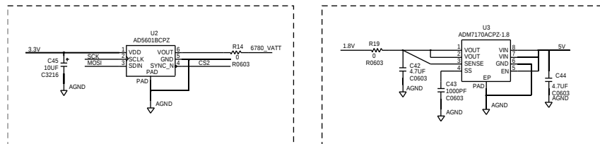
Figure 84. ADRF6780 Evaluation Board Schematic Page 2
