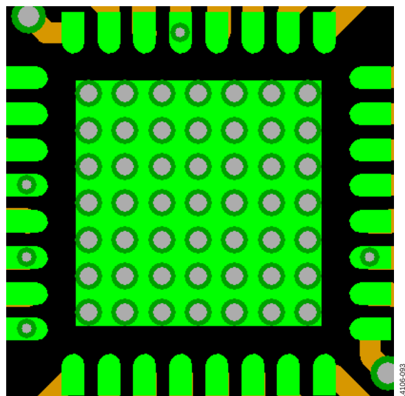
Figure 76. Evaluation Board Layout for the ADRF6780 Package
