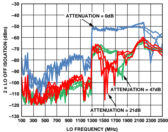
Figure 18. 2 x LO Off Isolation vs. LO Frequency, Attenuation, Supply, and Temperature
