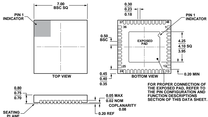
Figure 51. 48-Lead Lead Frame Chip Scale Package [LFCSP] 7 mm × 7 mm Body and 0.75 mm Package Height (CP-48-5)
