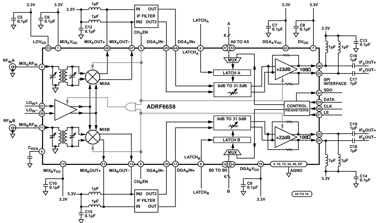
Figure 43. Basic Connections
