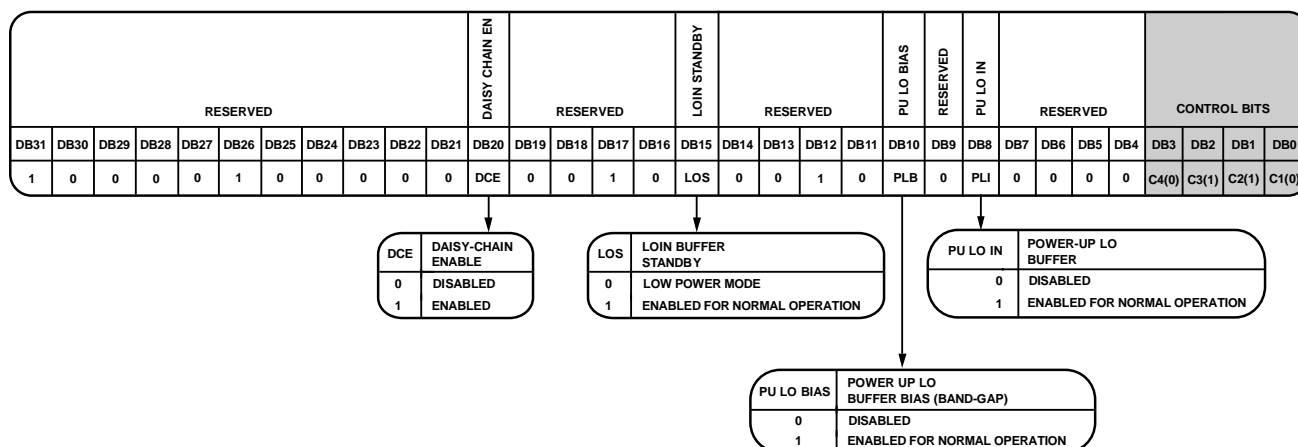
Figure 33. Register 6 (R6)
