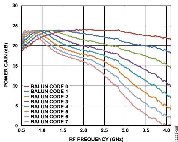
Figure 5. Power Gain vs. RF Frequency and Balun Codes
