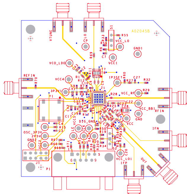
Figure 52. Evaluation Board Layout (Top)
