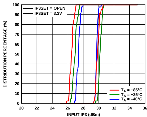
Figure 29. Input IP3
