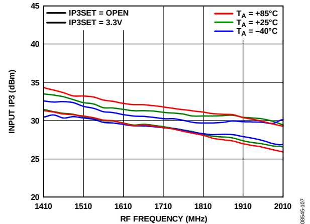
Figure 7. Input IP3 vs. RF Frequency
