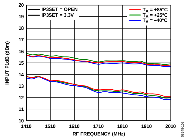
Figure 8. Input P1dB vs. RF Frequency
