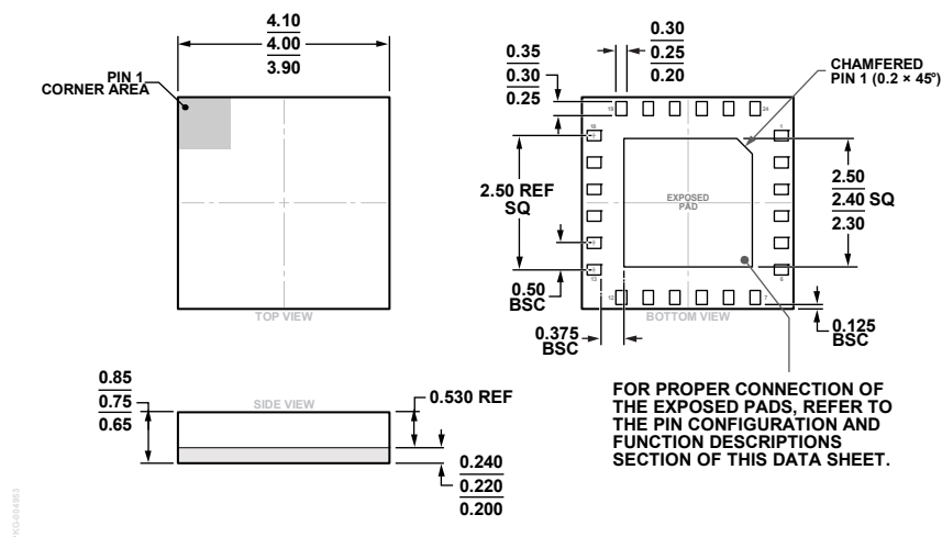
Figure 45. 24-Terminal Land Grid Array [LGA] 4 mm × 4 mm Body and 0.75 mm Package Height (CC-24-5)
