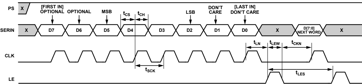
Figure 24. Serial Control Timing Diagram
