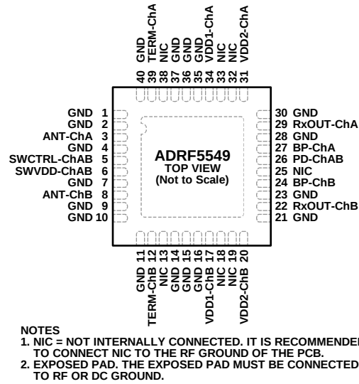
Figure 2. Pin Configuration
