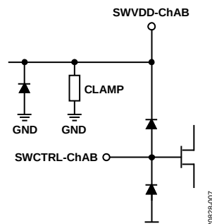
Figure 7. SWCTRL-ChAB and SWVDD-ChAB Interface Schematic
