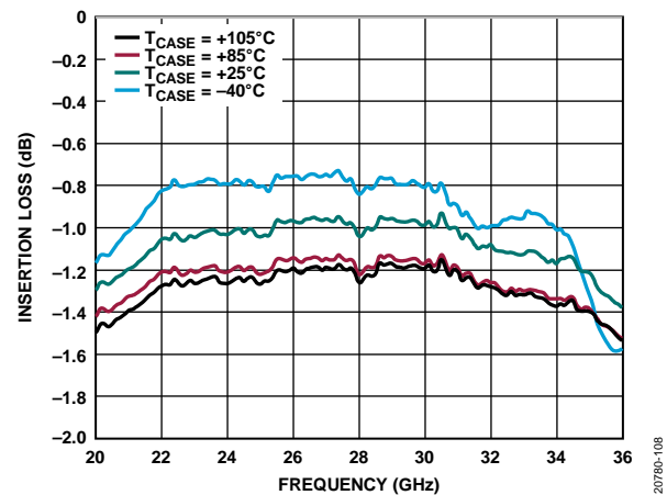
Figure 8. Insertion Loss vs. Frequency, RF1 Selected
