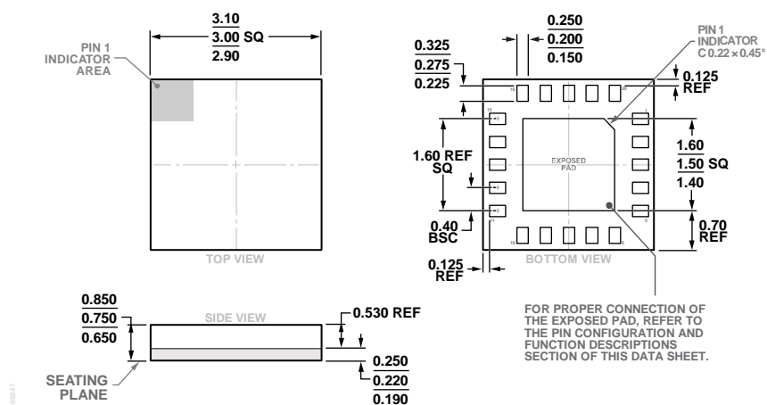
Figure 19. 20-Terminal Land Grid Array [LGA] 3 mm × 3 mm Body and 0.75 mm Package Height (CC-20-9)
