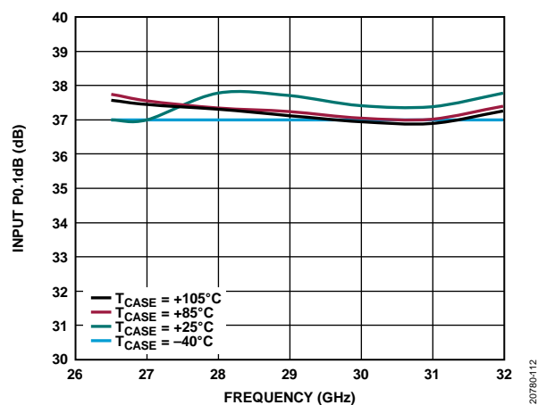
Figure 12. Input P0.1dB vs. Frequency, RF2 Selected
