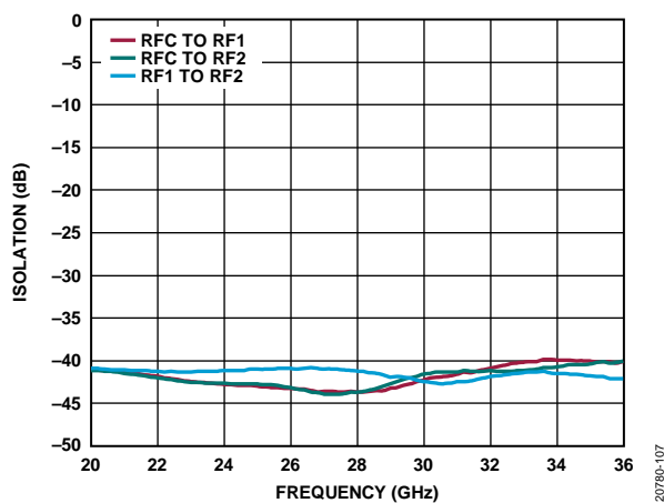
Figure 7. Isolation vs. Frequency
