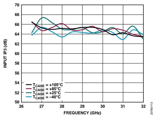
Figure 13. Input IP3 vs. Frequency, RF2 Selected
