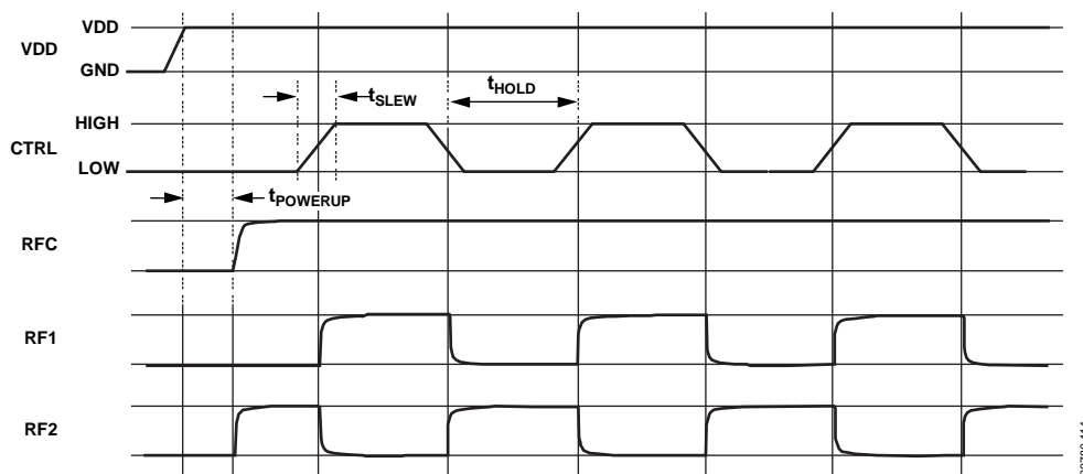
Figure 14. Timing Requirements
