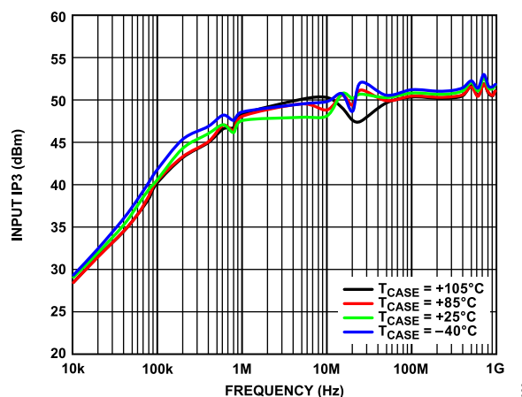
Figure 22. Input IP3 vs. Frequency over Various Temperatures (Low Frequency Detail)
