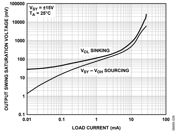
Figure 28. Output Swing Saturation Voltage vs. Load Current
