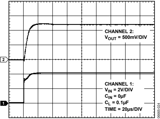
Figure 22. ADR827 Turn-On Response
