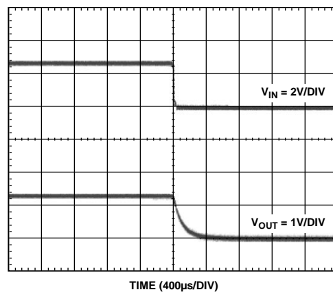
Figure 6. Turn Off Time
