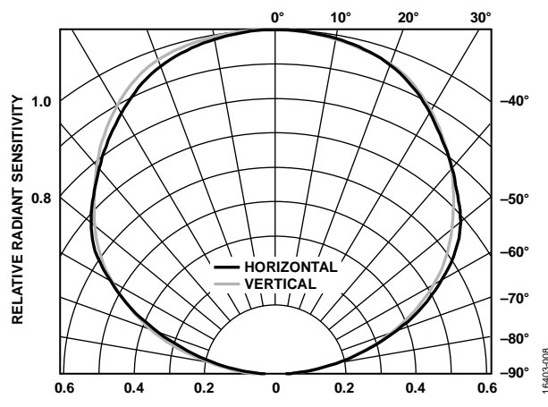
Figure 8. Relative Radiant Sensitivity vs. Angular Displacement
