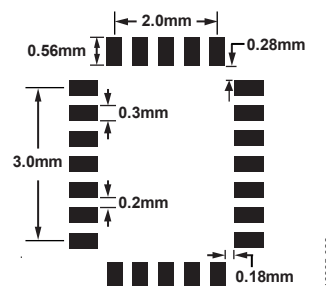
Figure 32. Land Pattern
