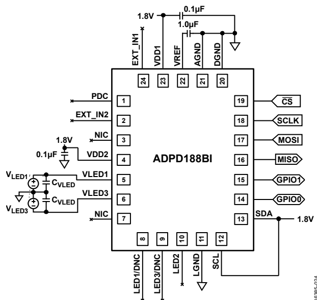
Figure 30. SPI Mode Connection Diagram
