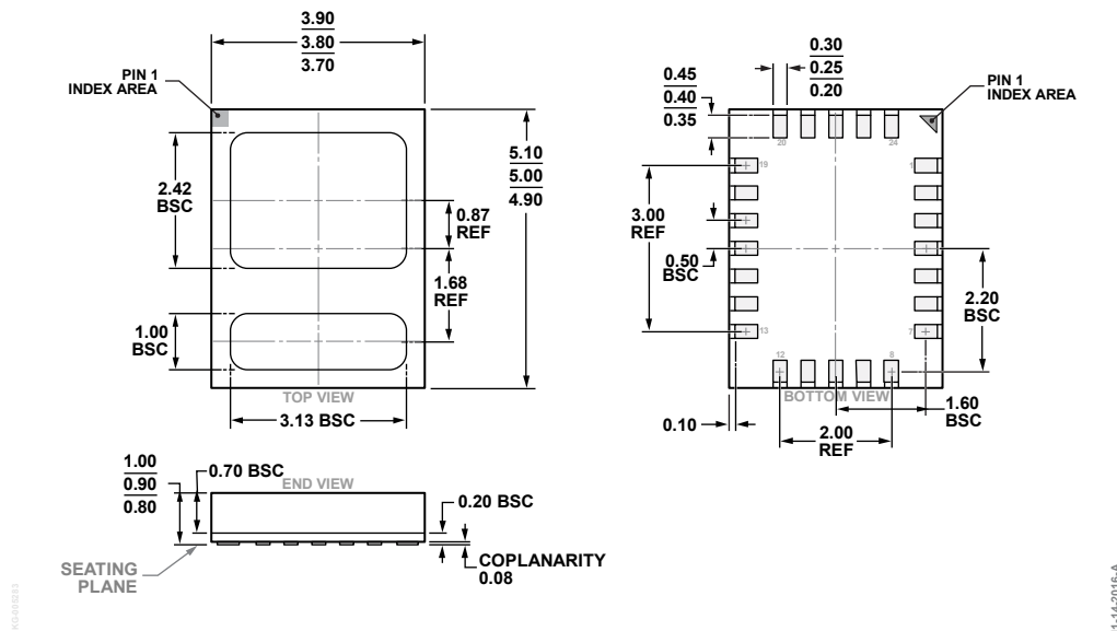
Figure 46. 24-Terminal Chip Array Small Outline No Lead Cavity [LGA_CAV] 3.80 mm × 5.00 mm Body and 0.9 mm Package Height (CE-24-1) Dimensions shown in millimeters
