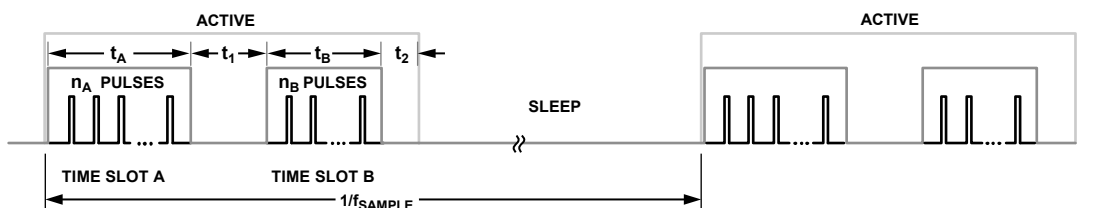
Figure 21. Time Slot Timing Diagram
