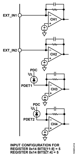
Figure 22. PD1 to PD4 Connection
