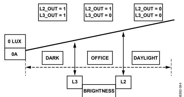
Figure 40. Light Sensor Modes Based on the Detected Ambient Light Level
