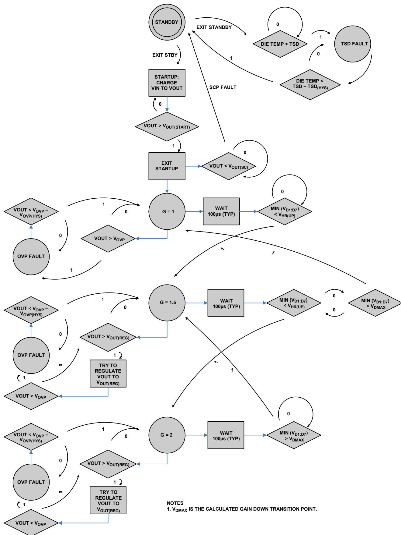
Figure 47. Fault State Machine
