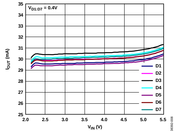
Figure 9. Typical Diode Matching vs. V_{IN}
