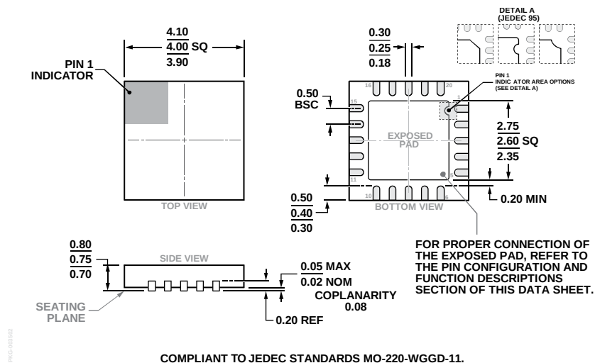
Figure 51. 20-Lead Lead Frame Chip Scale Package [LFCSP] 4 mm × 4 mm Body and 0.75 mm Package Height (CP-20-8)
