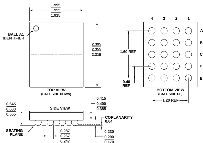
Figure 53. 20-Ball Wafer Level Chip Scale Package [WLCSP] (CB-20-6)
