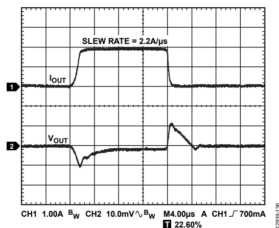
Figure 34. Load Transient Response, I_{\text{LOAD}} = 100\text{ mA} to 2\text{ A} , V_{\text{OUT}} = 3.3\text{ V} , V_{\text{IN}} = 4.0\text{ V} , C_{\text{OUT}} = 22\mu\text{F} , Channel 1 = I_{\text{OUT}} , Channel 2 = V_{\text{OUT}}
