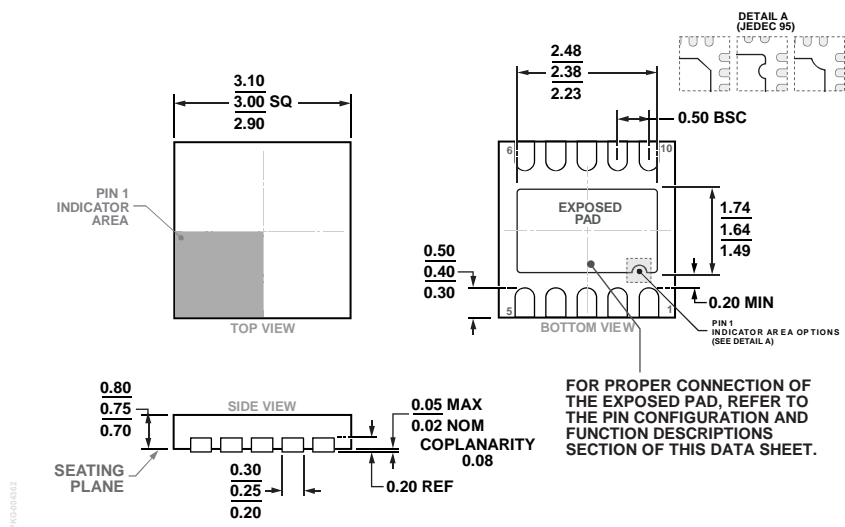
Figure 64. 10-Lead Lead Frame Chip Scale Package [LFCSP] 3 mm × 3 mm Body and 0.75 mm Package Height (CP-10-9)
