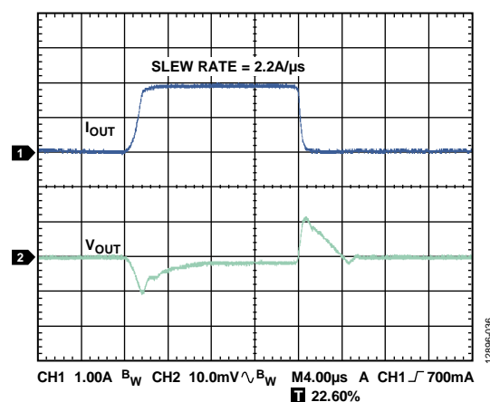
Figure 34. Load Transient Response, I_{\text{LOAD}} = 100\text{ mA} to 2 A, V_{\text{OUT}} = 3.3\text{ V} , V_{\text{IN}} = 4.0\text{ V} , C_{\text{OUT}} = 22\mu\text{F} , Channel 1 = I_{\text{OUT}} , Channel 2 = V_{\text{OUT}}
