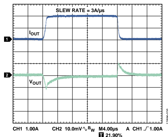
Figure 33. Load Transient Response, I_{\text{LOAD}} = 100\text{ mA} to 2 A, V_{\text{OUT}} = 3.3\text{ V} , V_{\text{IN}} = 4.0\text{ V} , Channel 1 = I_{\text{OUT}} , Channel 2 = V_{\text{OUT}}
