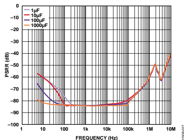
Figure 27. Power Supply Rejection Ratio (PSRR) vs. Frequency at Different C_{BYP} Values, V_{OUT} = 3.3\text{ V} , V_{IN} = 4.0\text{ V} , 1.2 A Load
