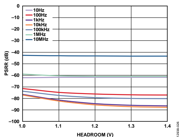
Figure 26. Power Supply Rejection Ratio (PSRR) vs. Headroom Voltage at Various Frequencies, V_{OUT} = 1.2\text{ V} , 1.2 A Load
