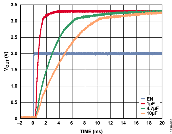
Figure 53. Typical Start-Up Behavior with C_{BYP} = 1 \mu\text{F}
