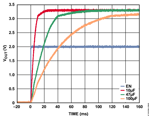
Figure 54. Typical Start-Up Behavior with C_{BYP} = 1 \mu\text{F} to 100 \mu\text{F}
