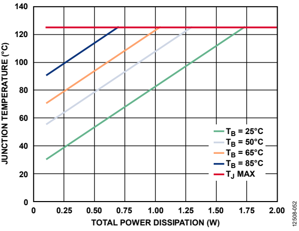
Figure 52. WLCSP Junction Temperature Rise, Different Board Temperatures
