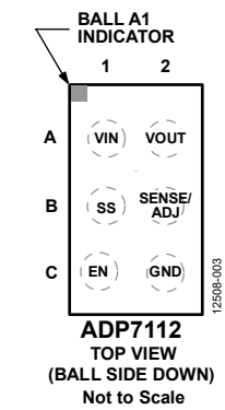
Figure 3. Pin Configuration
