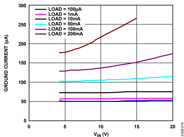
Figure 19. Ground Current vs. Input Voltage ( V_{IN} ), V_{OUT} = 3.3 V
