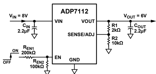
Figure 45. Typical EN Pin Voltage Divider
