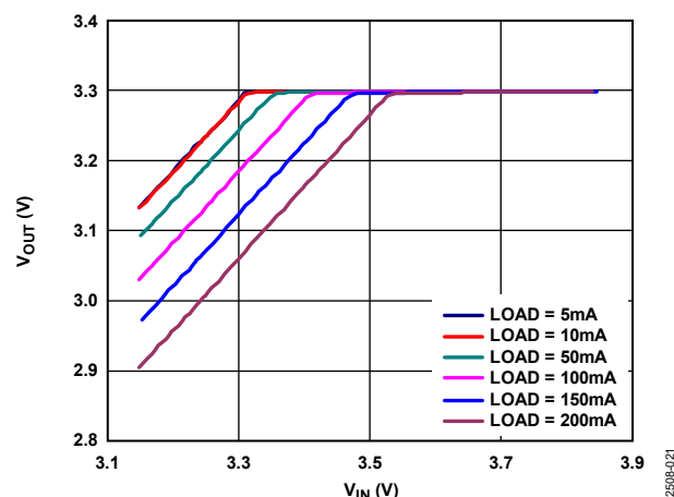
Figure 21. Output Voltage ( V_{OUT} ) vs. Input Voltage ( V_{IN} ) in Dropout, V_{OUT} = 3.3 V
