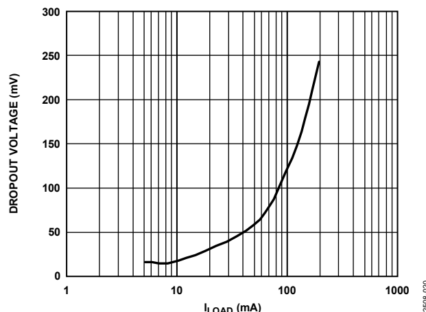
Figure 20. Dropout Voltage vs. Load Current ( I_{LOAD} ), V_{OUT} = 3.3 V
