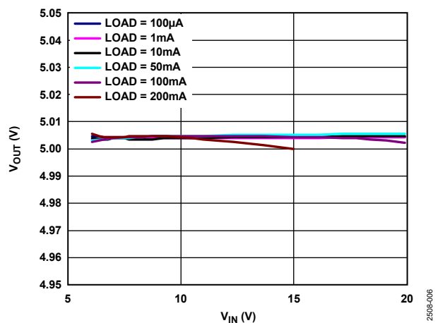
Figure 6. Output Voltage ( V_{OUT} ) vs. Input Voltage ( V_{IN} )
