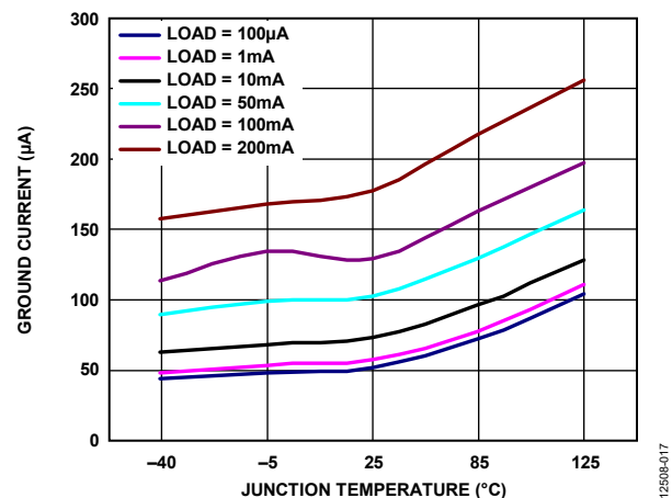
Figure 17. Ground Current vs. Junction Temperature, V_{OUT} = 3.3 V
