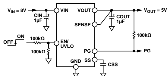
Figure 1. ADP7105 with Fixed Output Voltage, 5 V
