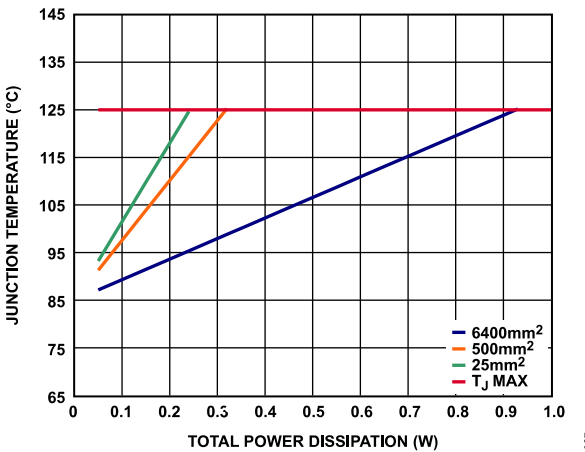
Figure 72. LFCSP, T_A = 85^\circ\text{C}
